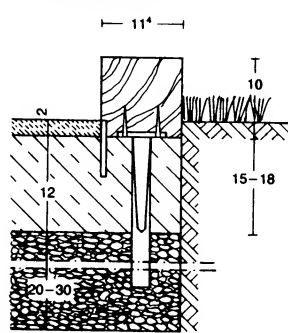
⑥ Circle edge board/shot put section A-B
